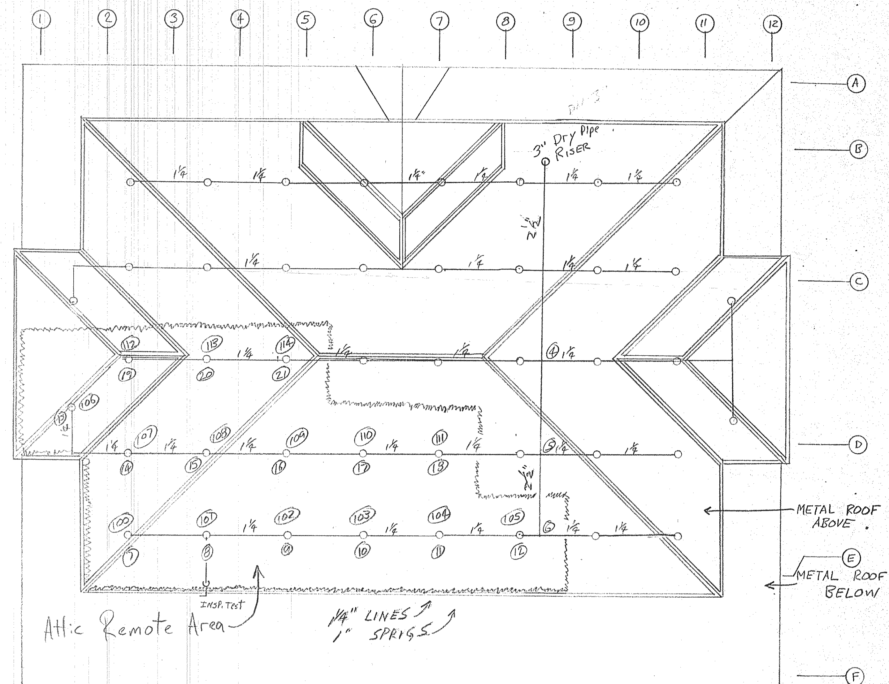
ROOF PLAN
