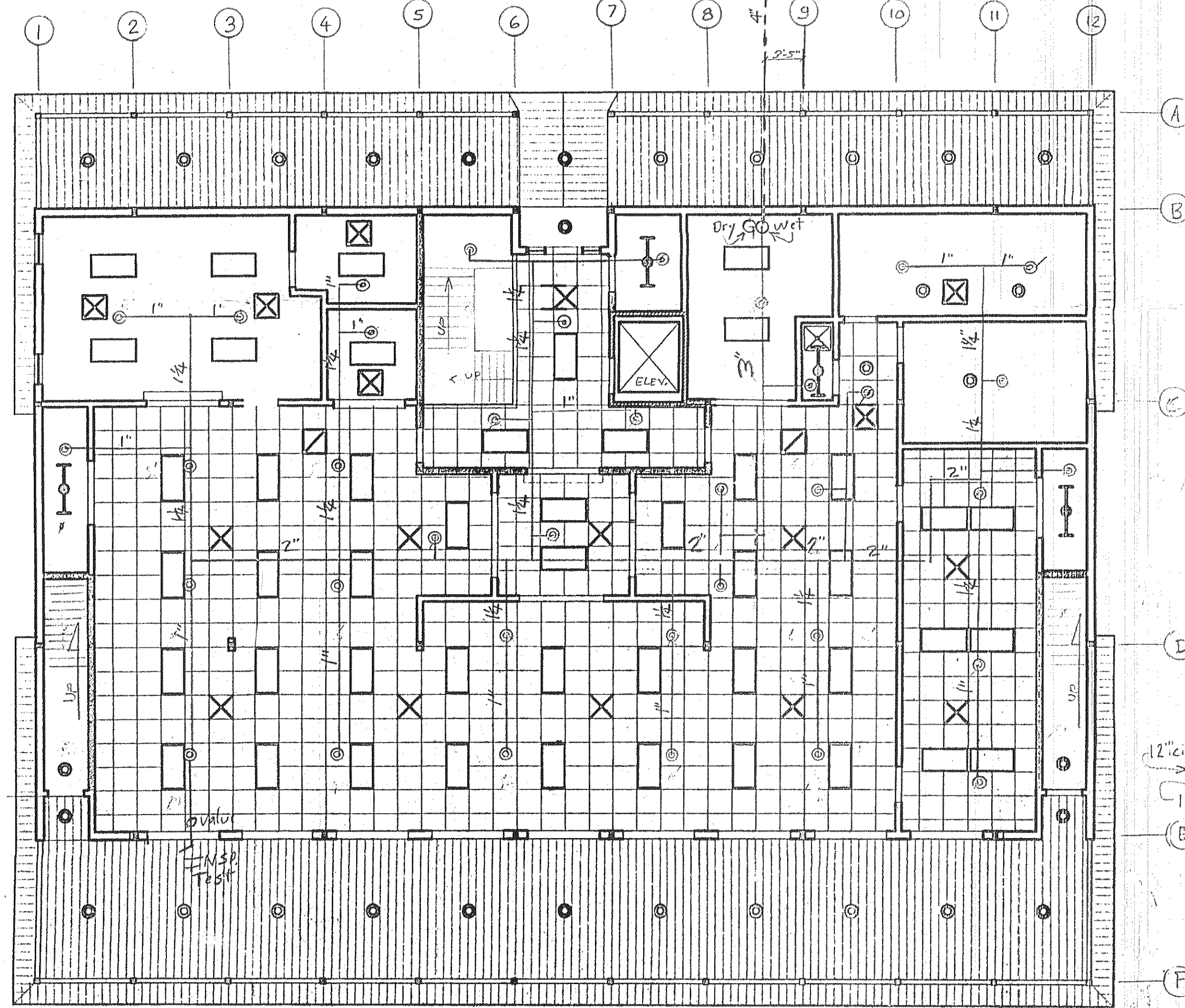
SECOND FLOOR REFLECTED CEILING PLAN SCALE: 1/8" = 1'-0"
