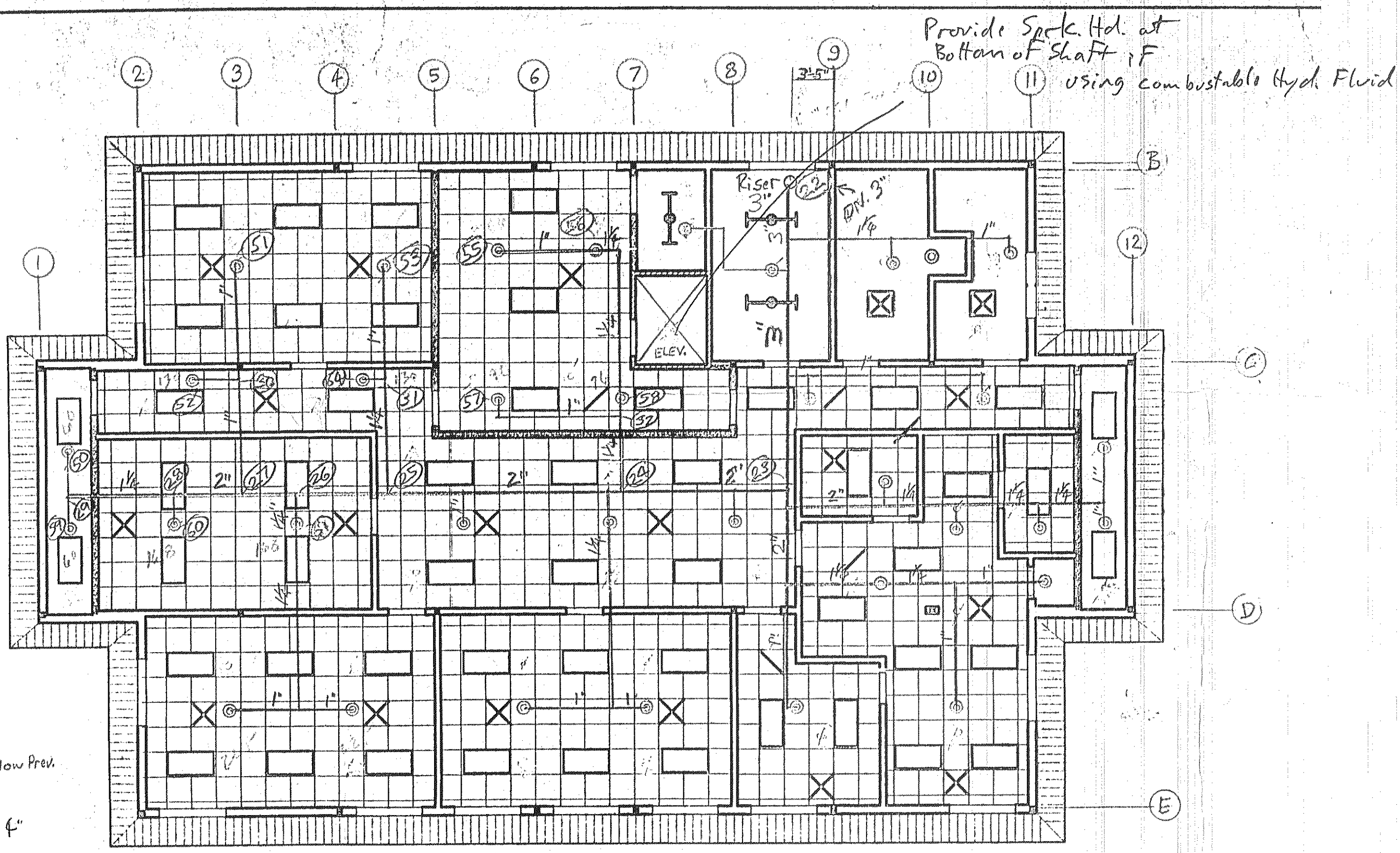
SECOND FLOOR REFLECTED CEILING PLAN SCALE: 1/8" = 1'-0"
